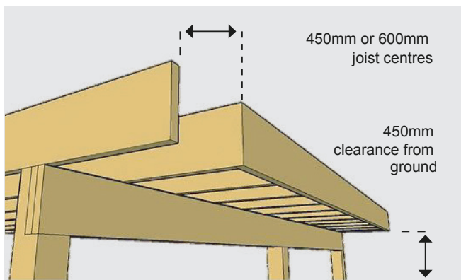
Above: Ventilation and clearance indicated
